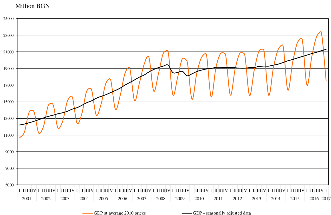
Figure 1. GDP by quarters for the period 2001 - 2017, at average 2010 prices
